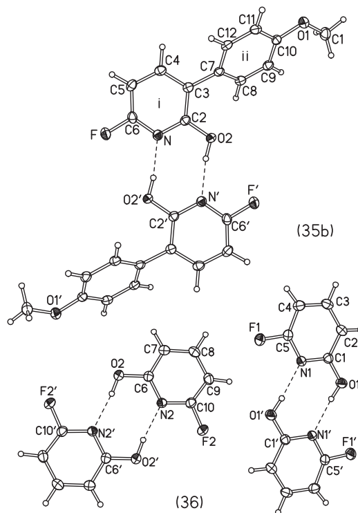
Figure 3. X-ray molecular structures of 35b and 36 , showing independent molecules, their inversion equivalents (primed) and hydrogen bonds (dashed lines). Interplanar angle i / ii 50.1°. Bond distances (Å): C(2)–O(2) 1.337(2), N–C(2) 1.339(2), N–C(6) 1.323(2), O(2)⋯N' 2.758(2), O(2)–H 0.92(2) in 35b ; C(1)–O(1) 1.330(1), N(1)–C(1) 1.342(1), N(1)–C(5) 1.320, C(6)–O(2) 1.335(1), N(2)–C(6) 1.342(1), N(2)–C(10) 1.323(1), O(1)⋯N(1') 2.735(1), O(1)–H 0.88(2), O(2)⋯N(2') 2.760(1), O(2)–H 0.89(2) in 36 indicate 2-hydroxypyridine tautomeric structures.
